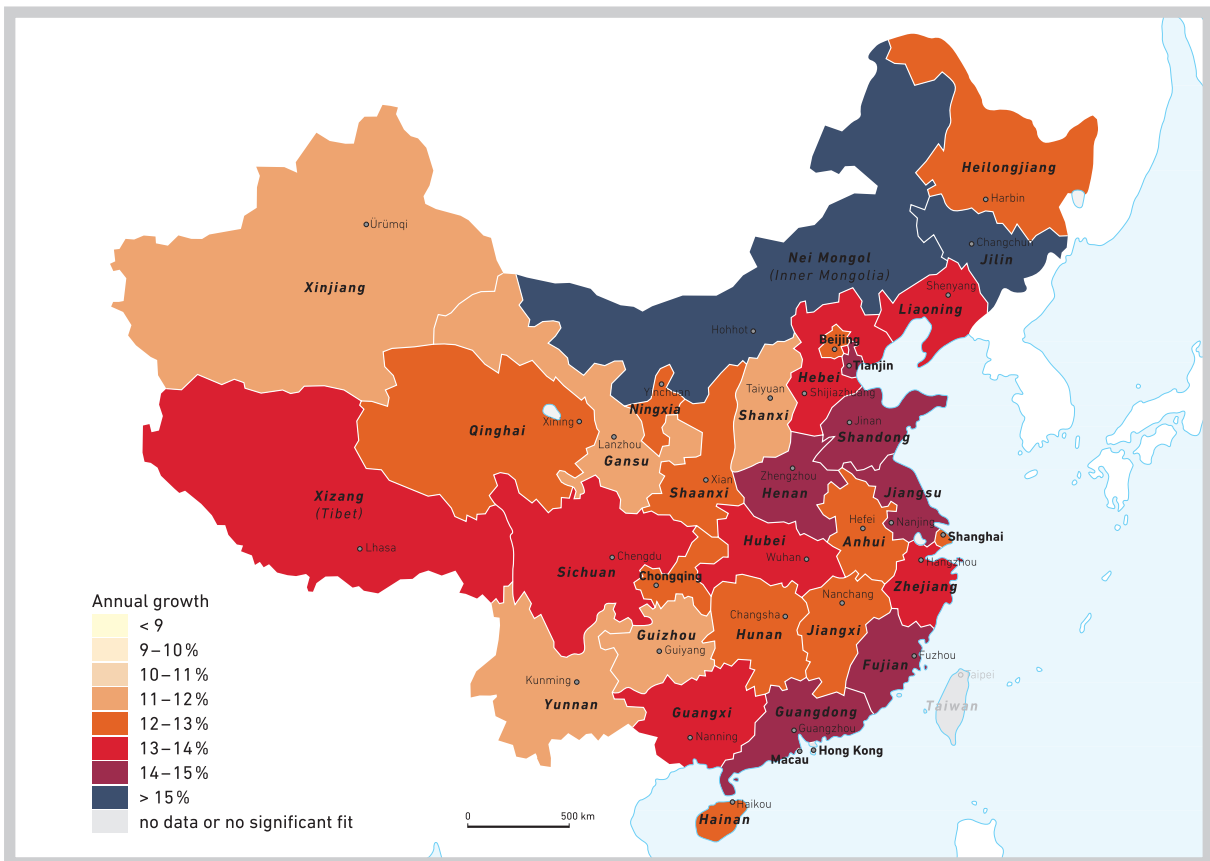
Figure 15: Annual growth 2008 by province
