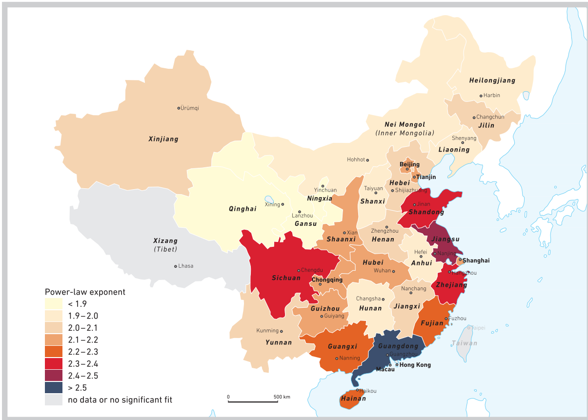
Figure 11: Power-law exponents for firm size measured in capital, by province, 2008, values as in Table 2
