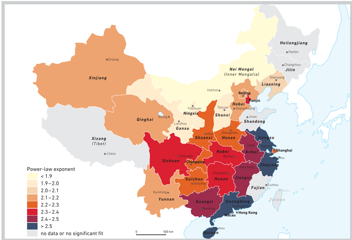
Figure 13: Power-law exponents for firm size measured in number of employees, by province, 2008, values as in Table 2
