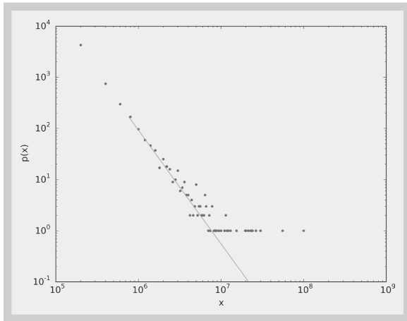
Figure 1: Firm size (measured in capital) distribution (probability density function), China, 2008
