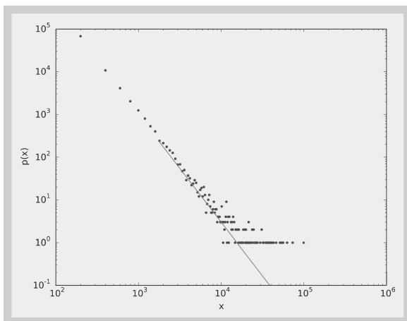
Figure 3: Firm size (measured in number of employees) distribution (probability density function), China, 2008
