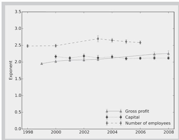
Figure 9: Development of power-law exponents for firm size in terms of capital, gross profits, and number of employees for Shanghai, 1998–2008, significant values only (KS test with 10 % threshold and log-likelihood ratio vs. lognormal and exponential fit).
