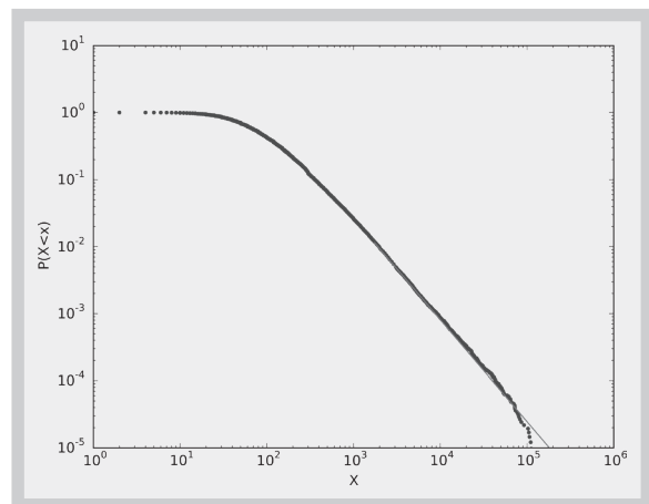
Figure 4: Survival function (complementary cumulative distribution function) for the firm size (measured in number of employees) distribution, China, 2008
