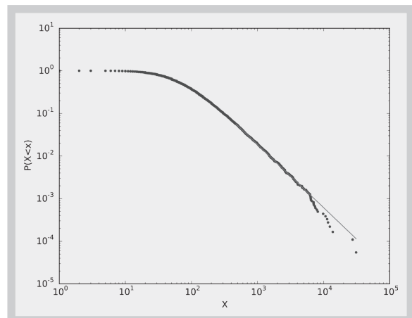
Figure 6: Survival function (complementary cumulative distribution function) for the firm size (measured in number of employees) distribution, Shanghai, 2008
